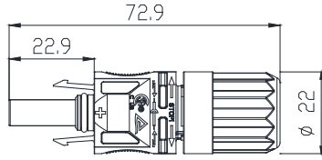
Female connector (+)
